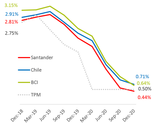
CLP Time Deposit Cost Evolution 1
